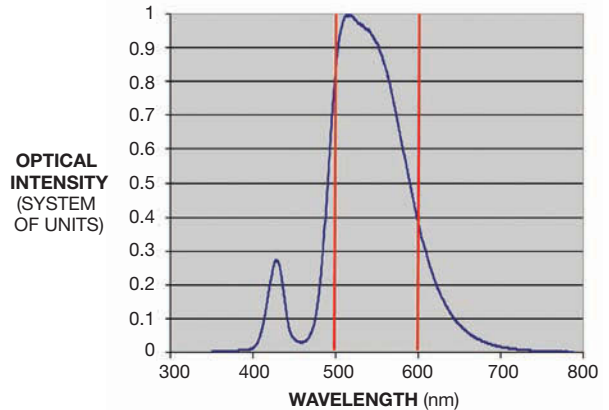
Figure 8 The built-in dichroics in a two- or three-channel architecture remove the overlapping color spectrum, resulting in approximately 40% higher white-lumen output.
