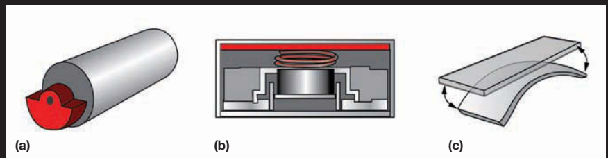
Figure A Haptics displays rely on actuators to give a touchscreen the ability to touch back. The main types of actuators in haptics are eccentric rotating masses (a), linear resonant actuators (b), and piezoelectric actuators (c).
