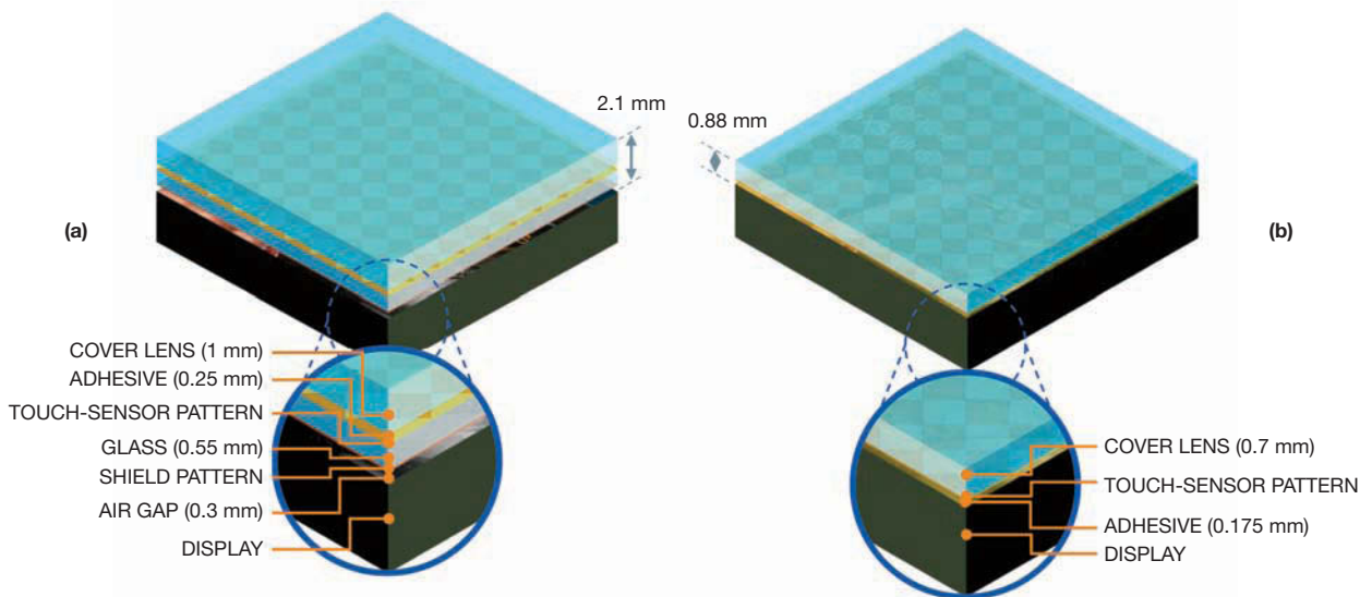
Figure 1 The touchscreen stack has an ITO shield (a). The lack of such a shield means fewer layers to reduce thickness and increase display brightness but can make for LCD-noise problems (b).
