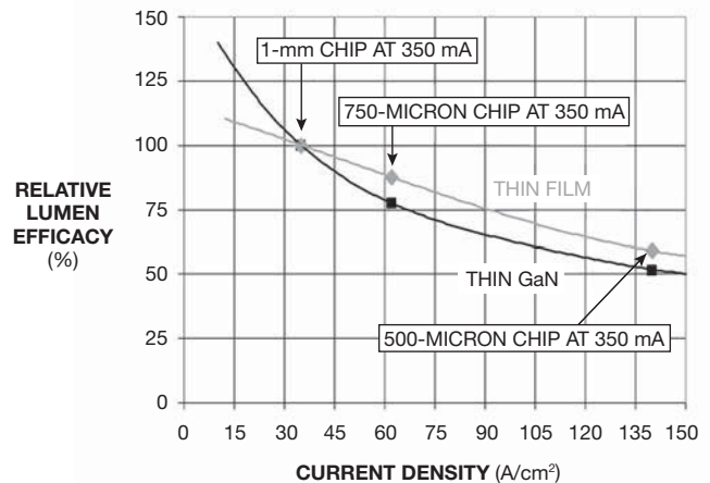
Figure 3 The relative efficacy, normalized to 100% at 350 mA/mm 2 , for ThinFilm and ThinGaN chips, decreases with increasing current density at 350 mA for the standard chip sizes: 500 microns, 750 microns, and 1 mm, or 20, 30, and 40 mil.
