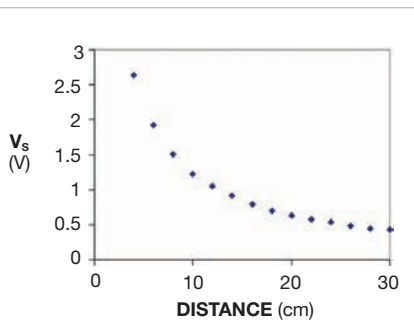
Figure 1 The analog voltage directly from the sensor is not linear with the distance.
