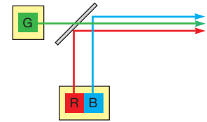
Figure 6 Combining red and blue in one device and green in a separate package is the basis for a two-channel configuration.
